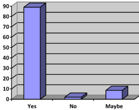
Fig. 4. Survey Analysis
